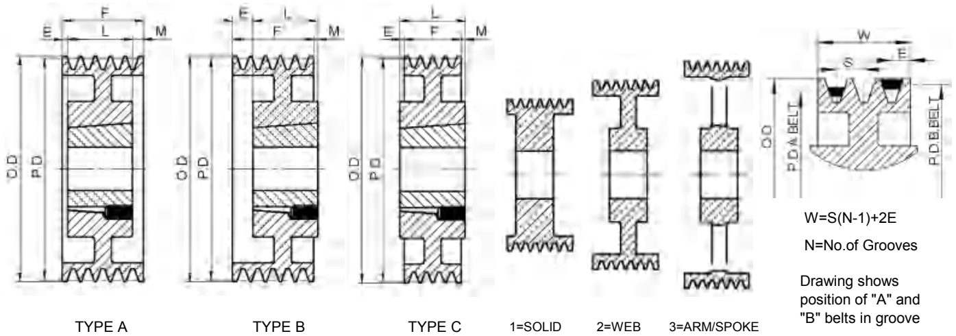
Combination Groove Dimensions
