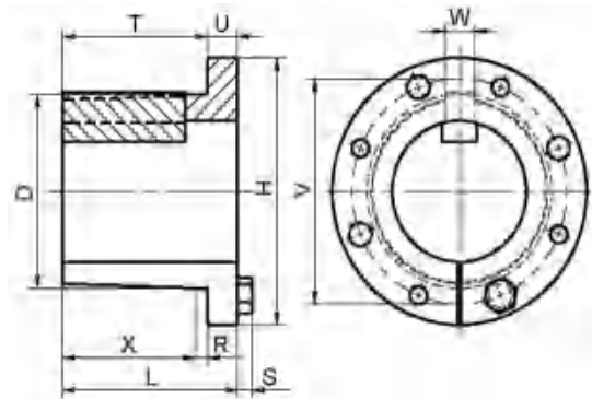
"W" AND "Y" BUSHINGS
