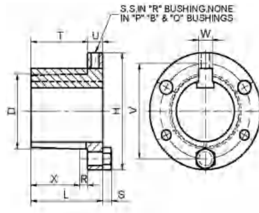
"P", "B", "Q" & "R" BUSHINGS
