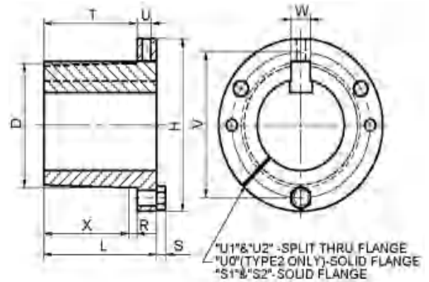
"S" & "U" BUSHINGS
