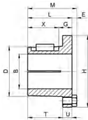
Bushing Dimension
