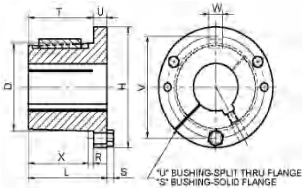
"S" & "U" BUSHINGS
