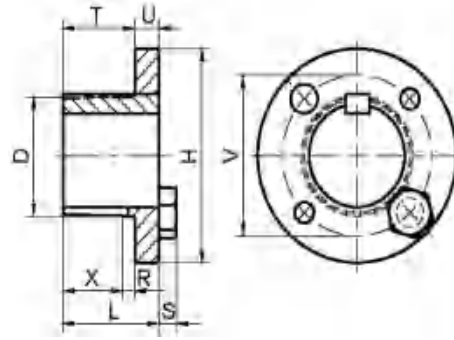
G & H BUSHINGS
